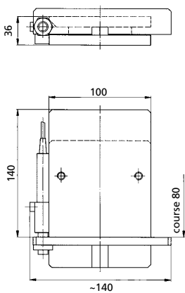
ST 10/ST 10 P (course 80 mm)
