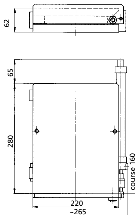
ST 140 P (course 160 mm)
