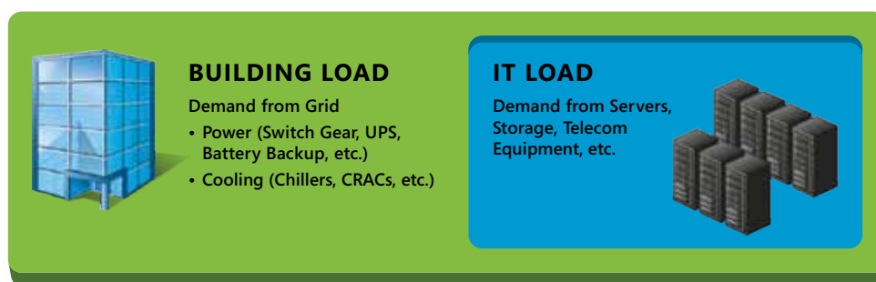
FIGURE 1: PUE = \text{TOTAL FACILITY POWER} / \text{IT EQUIPMENT POWER}
