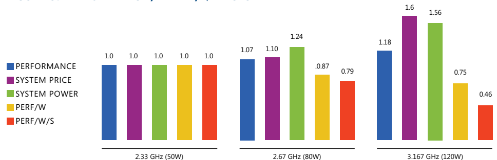
FIGURE 3: PERFORMANCE / WATT / $ AT SYSTEM LEVEL
